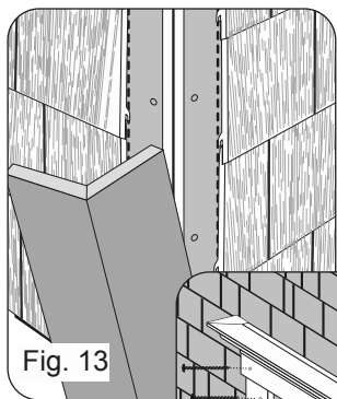
Cortex® Hidden Fastening System
